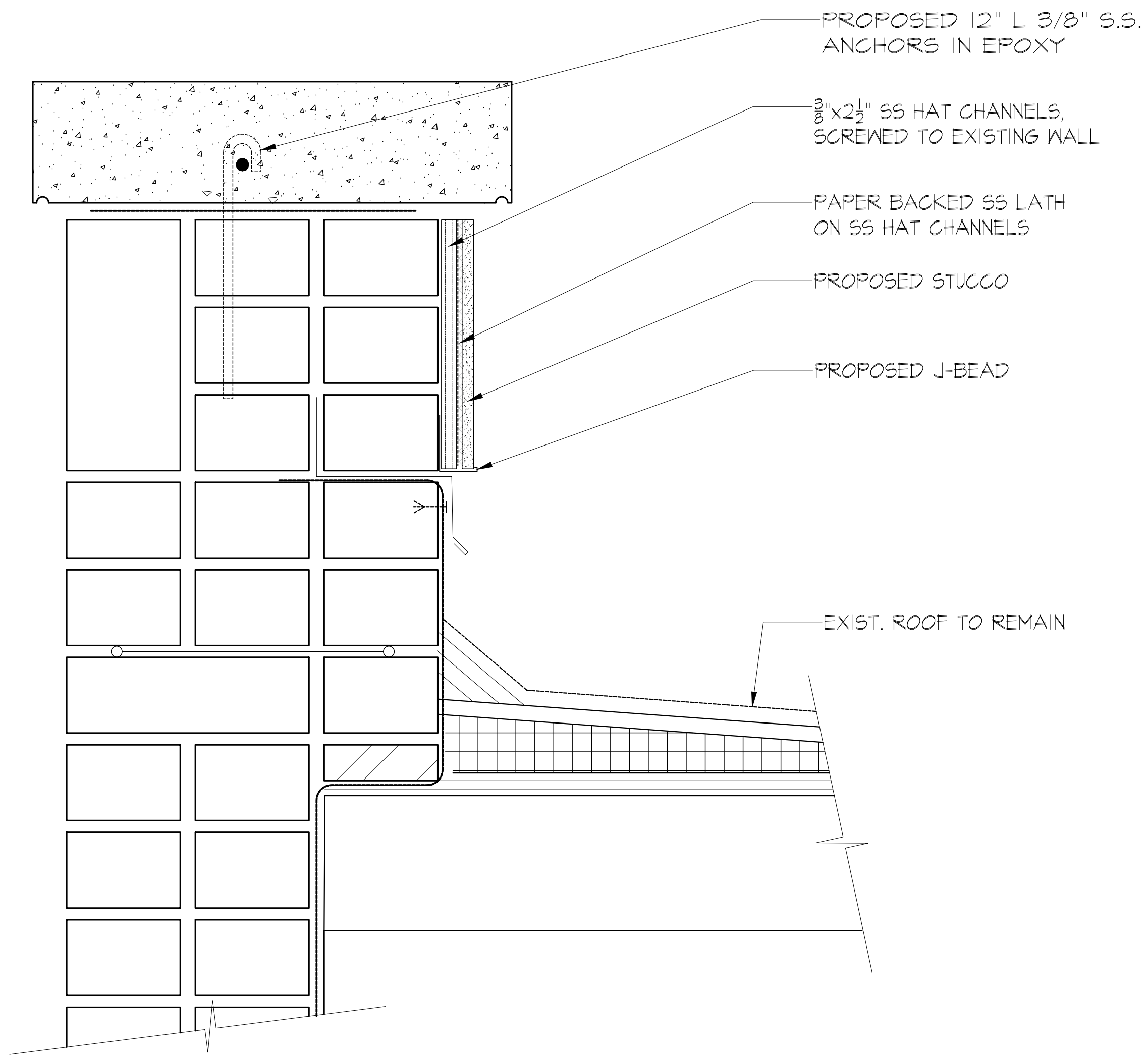
1 NORTH PARAPET WALL REPAIR DETAIL A-206 SCALE: NTS
