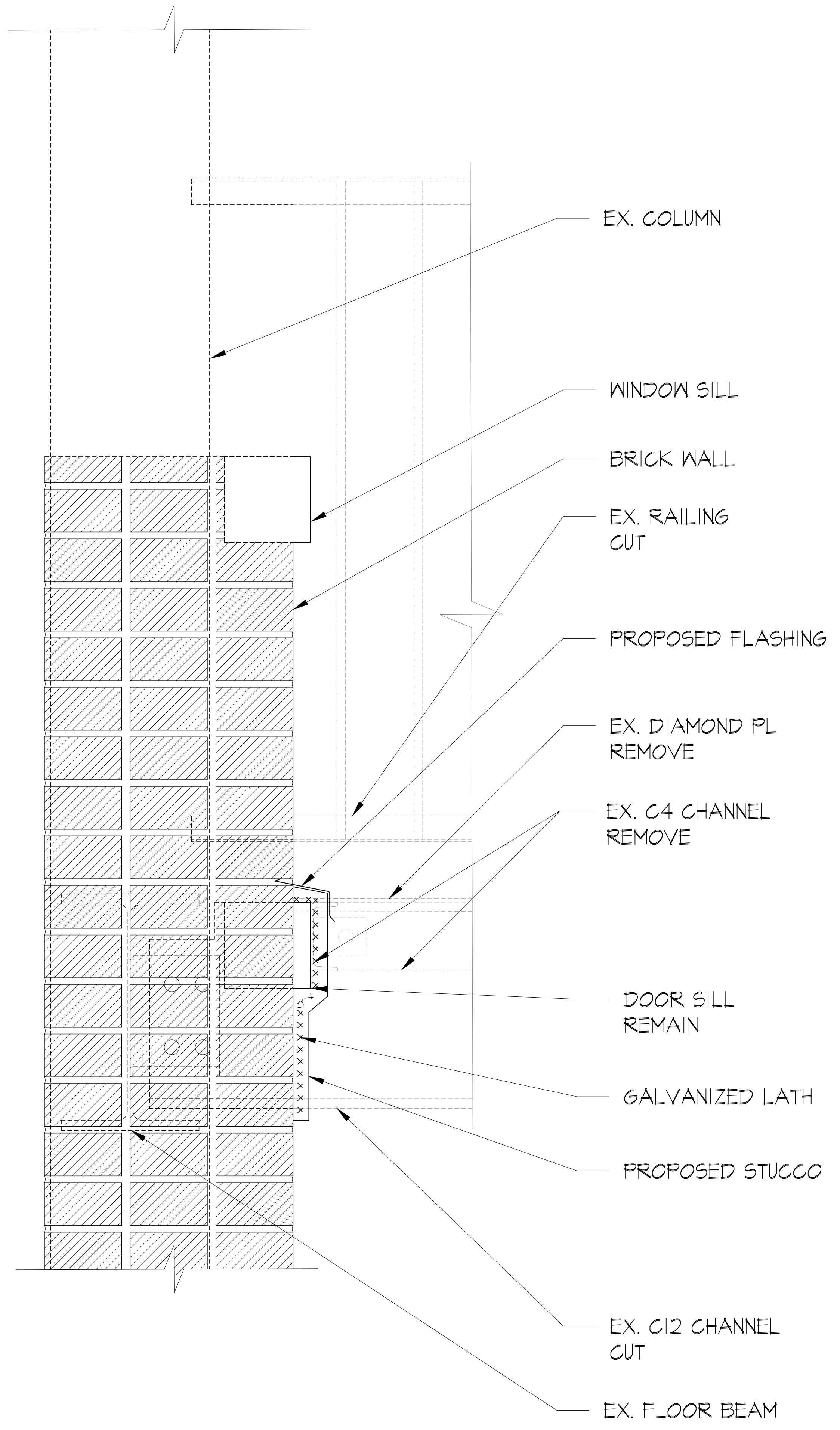
1 REMOVAL DETAIL - OPTION 1 A-203 SCALE:NTS
