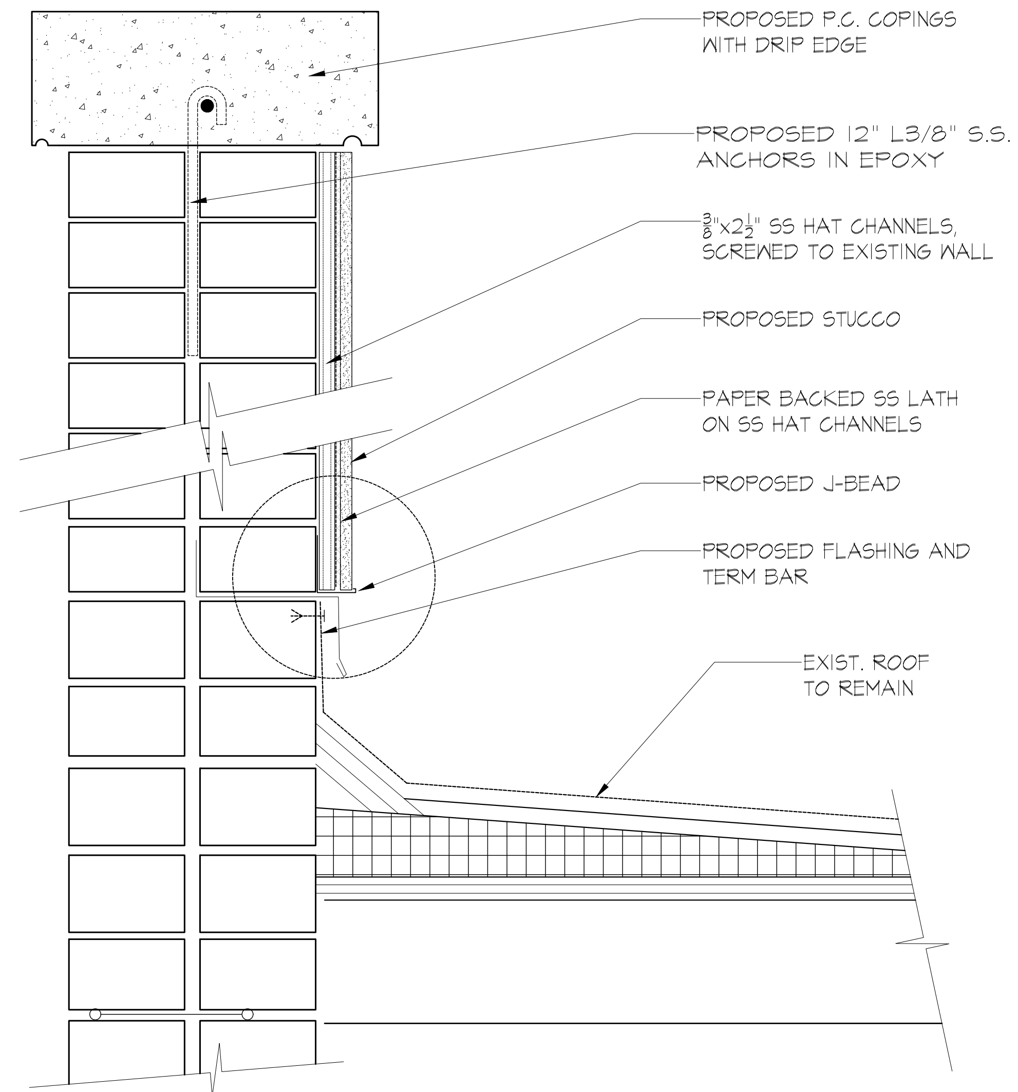
2 SOUTH & WEST PARAPET WALL REPAIR A-206 SCALE: NTS
