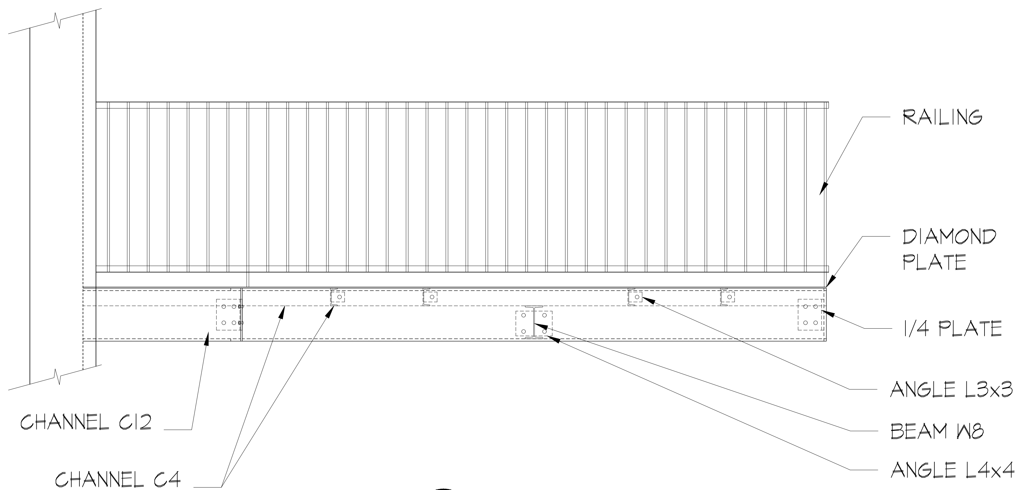
2 BALCONY TYP, 2 (WEST) - ELEVATION A-202 SCALE:NTS
