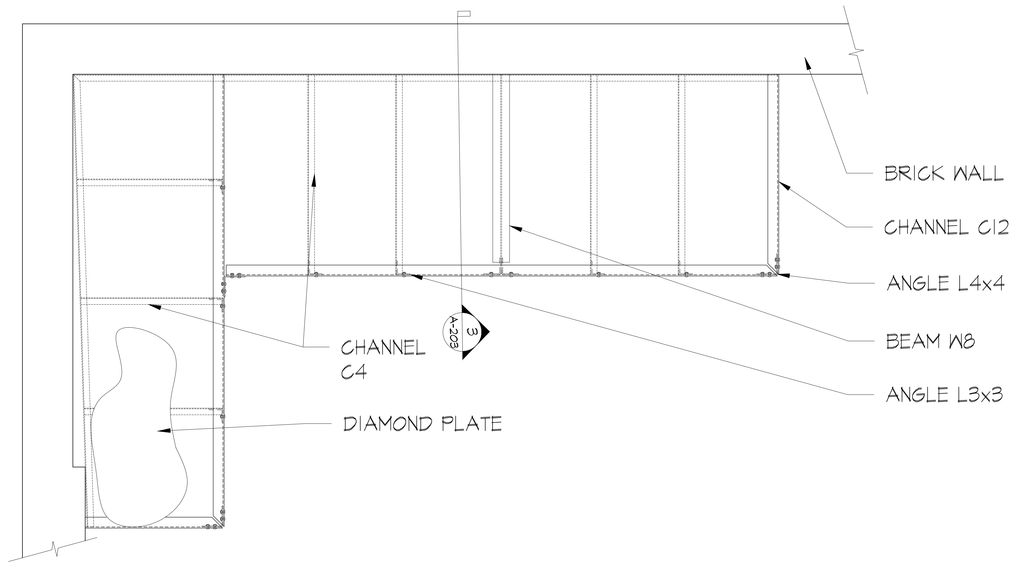
1 BALCONY TYP, 2 (WEST) - PLAN A-202 SCALE:NTS
