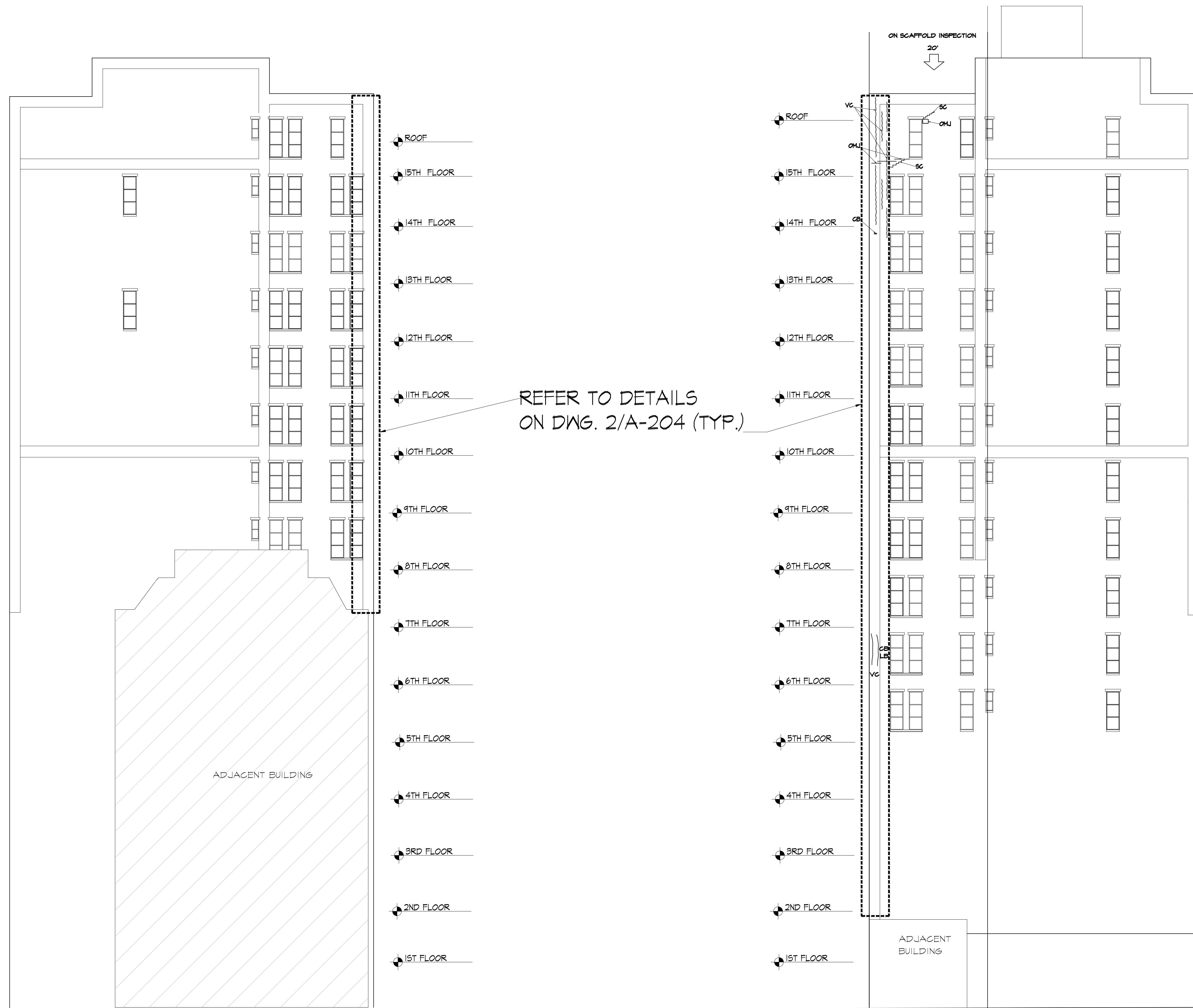
1 EAST ELEVATION A-102 SCALE:NTS
