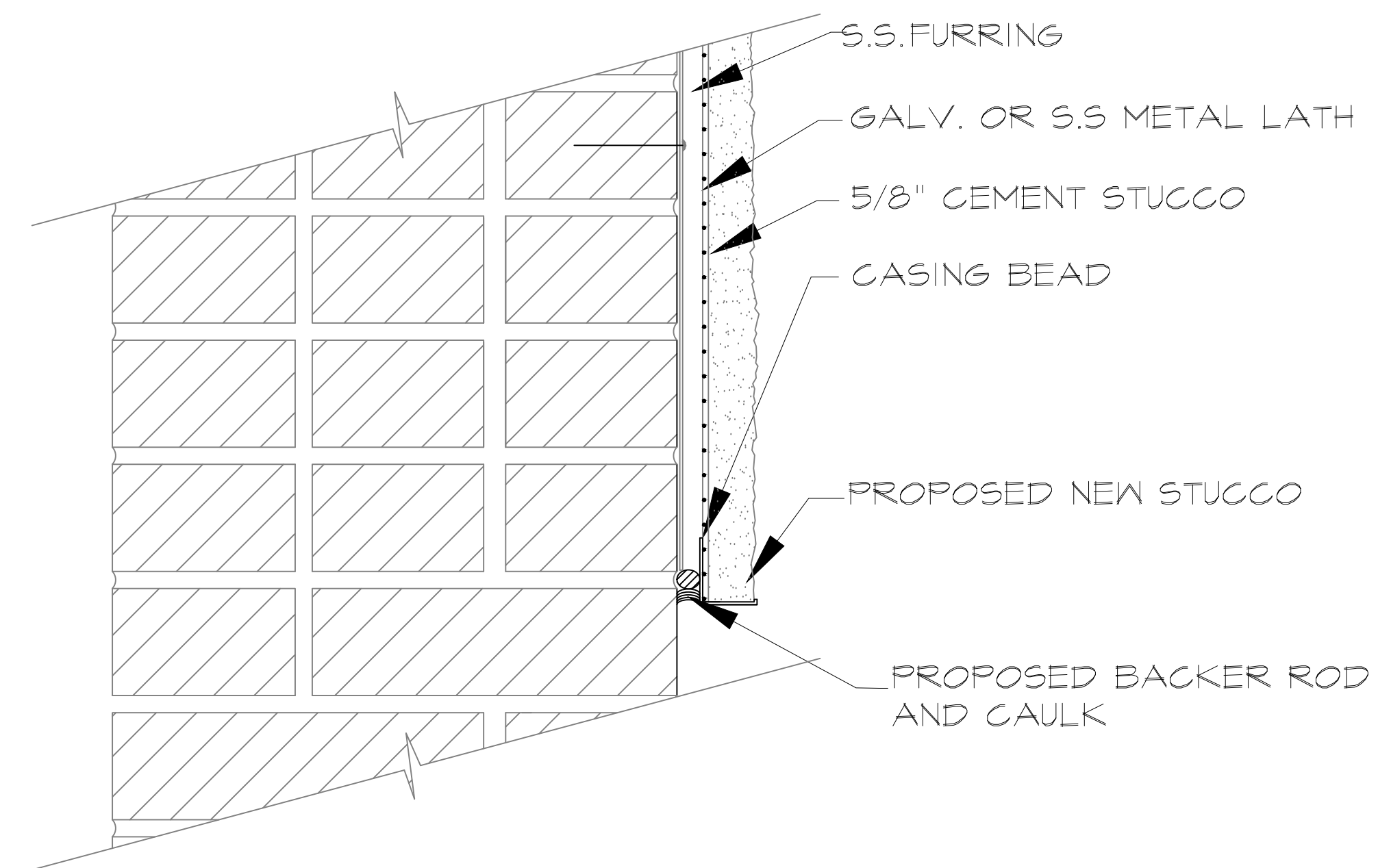
2 SOUTH & WEST PARAPET WALL REPAIR A-206 SCALE: NTS
