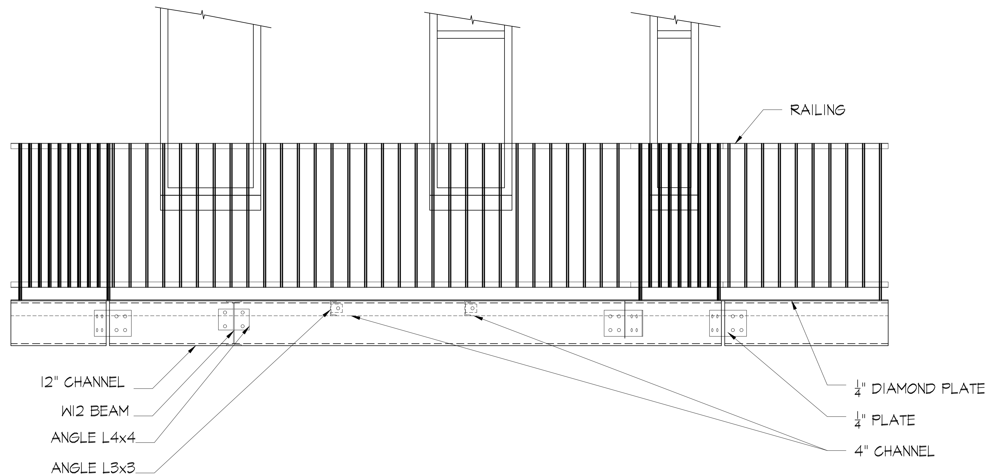
2 ELEVATION, BALCONY TYP, I (SOUTH EAST) - EXISTING CONDITIONS A-200 SCALE: 3/4" = 1'-0"
