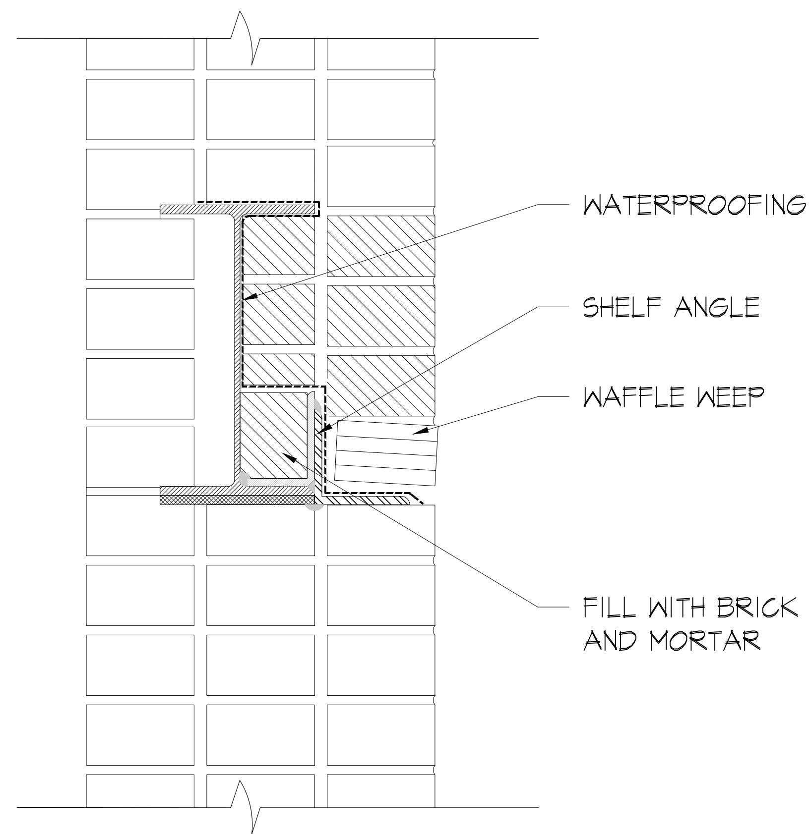
2 SPANDREL BEAM REINFORCEMENT DETAIL A-205 SCALE: 3"=1'-0"
