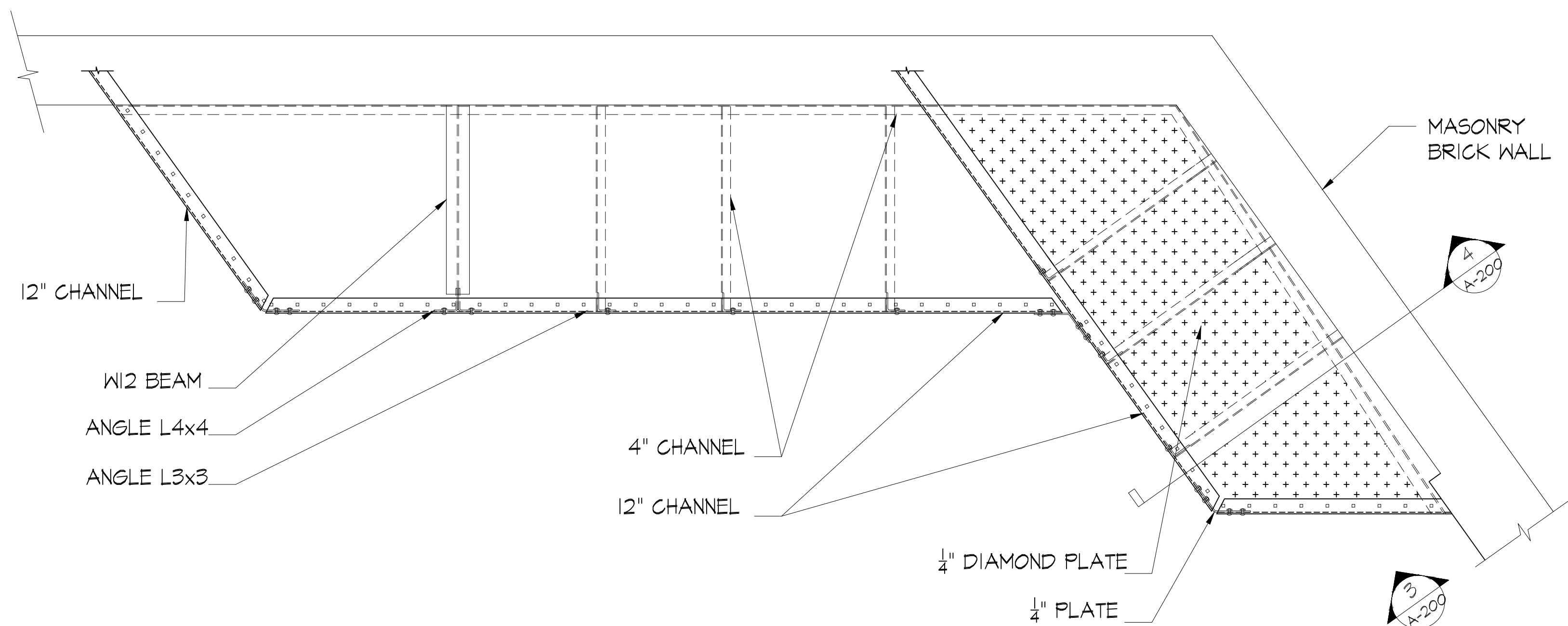
1 PLAN- BALCONY TYP, I (SOUTH EAST) - EXIST. CONDITIONS A-200 SCALE: 3/4" = 1'-0"
