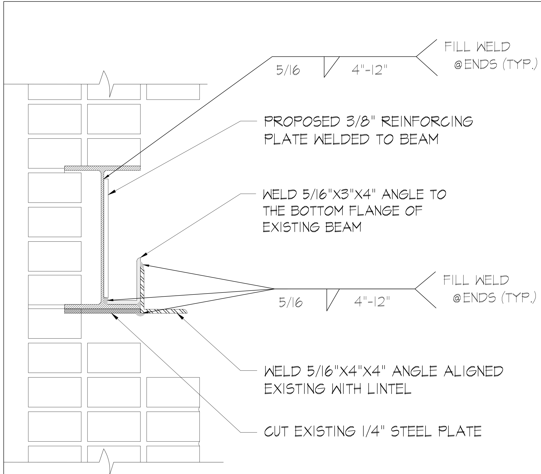
1 SPANDREL BEAM REINFORCEMENT DETAIL A-205 SCALE: 3"=1'-0"
