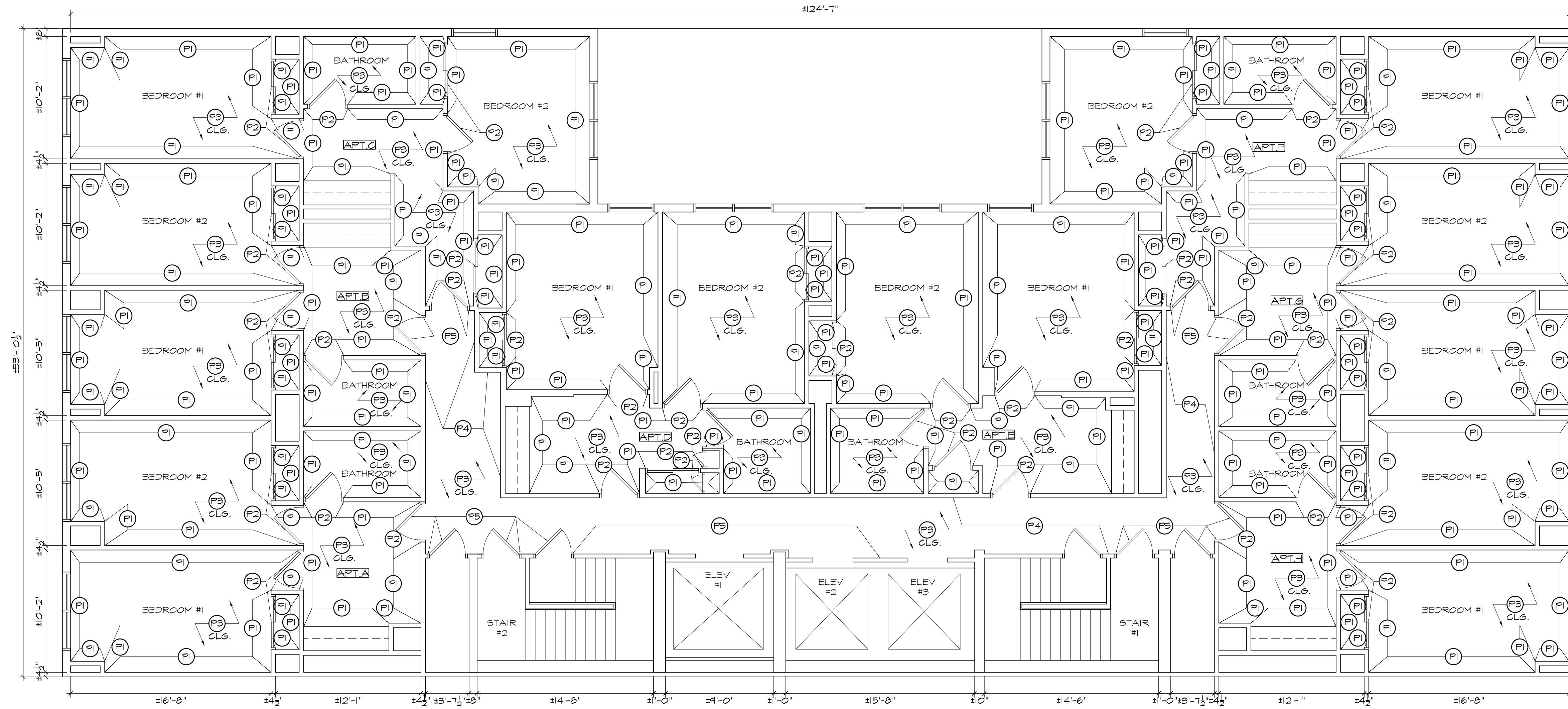
1 TYPICAL FINISH PLAN FOR FLOORS 2-6 A-300 SCALE: 3/16" = 1'-0"
