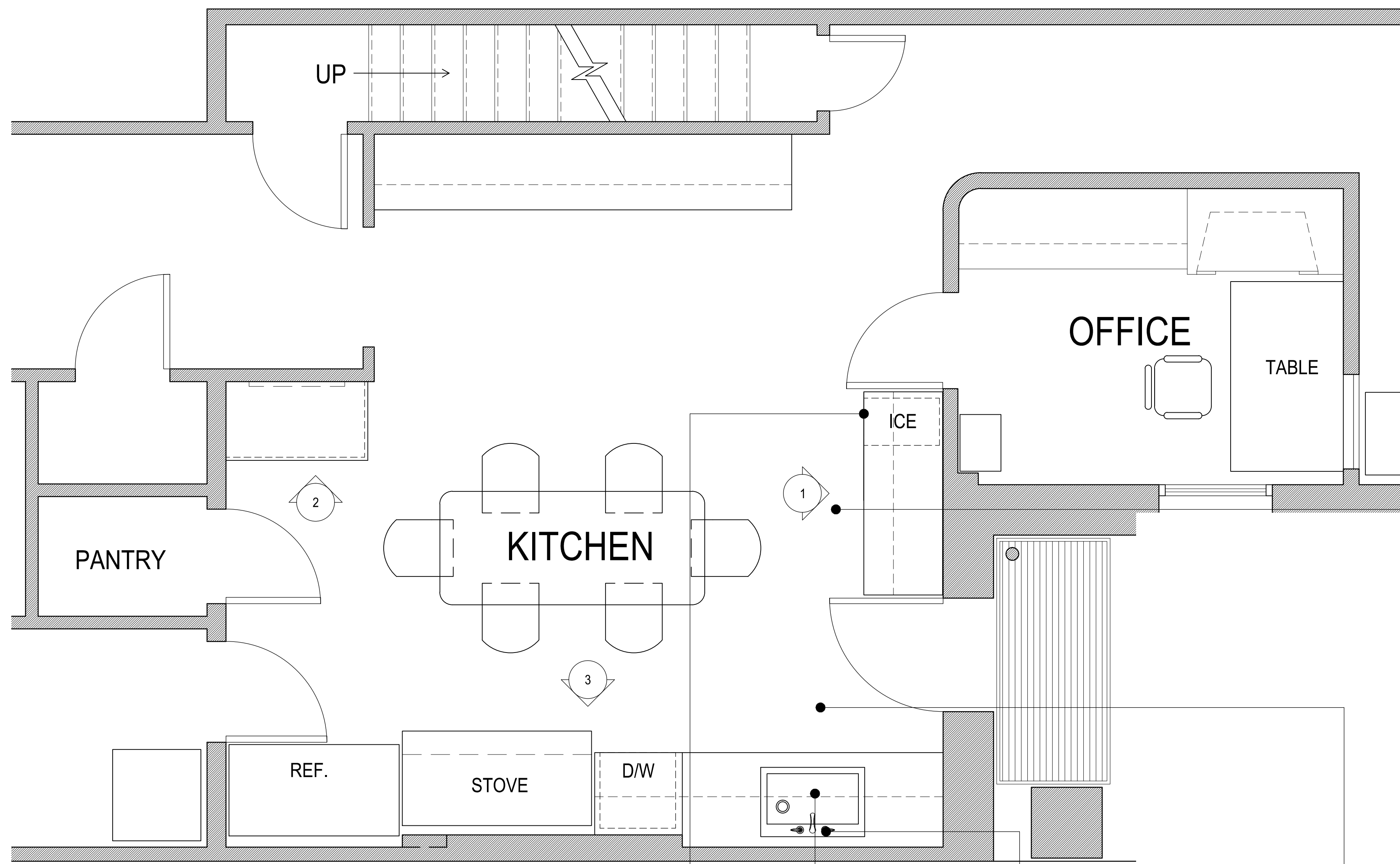
FLOOR PLAN
